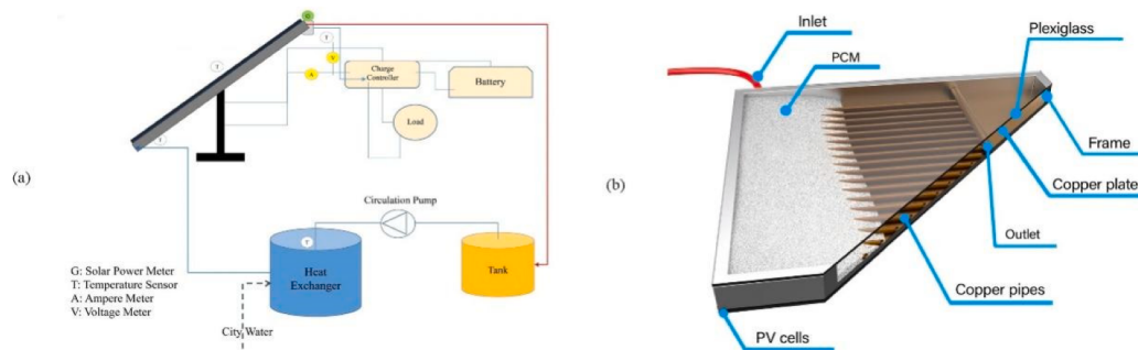
Fig. 2. PVT panel schematic and its main components [95] (Reprinted with permission from Elsevier).
